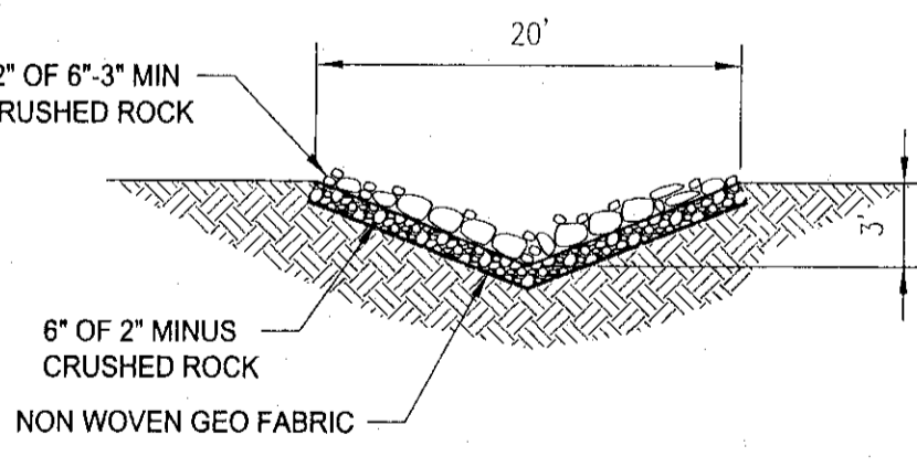
ARMORED V-DITCH NTS
