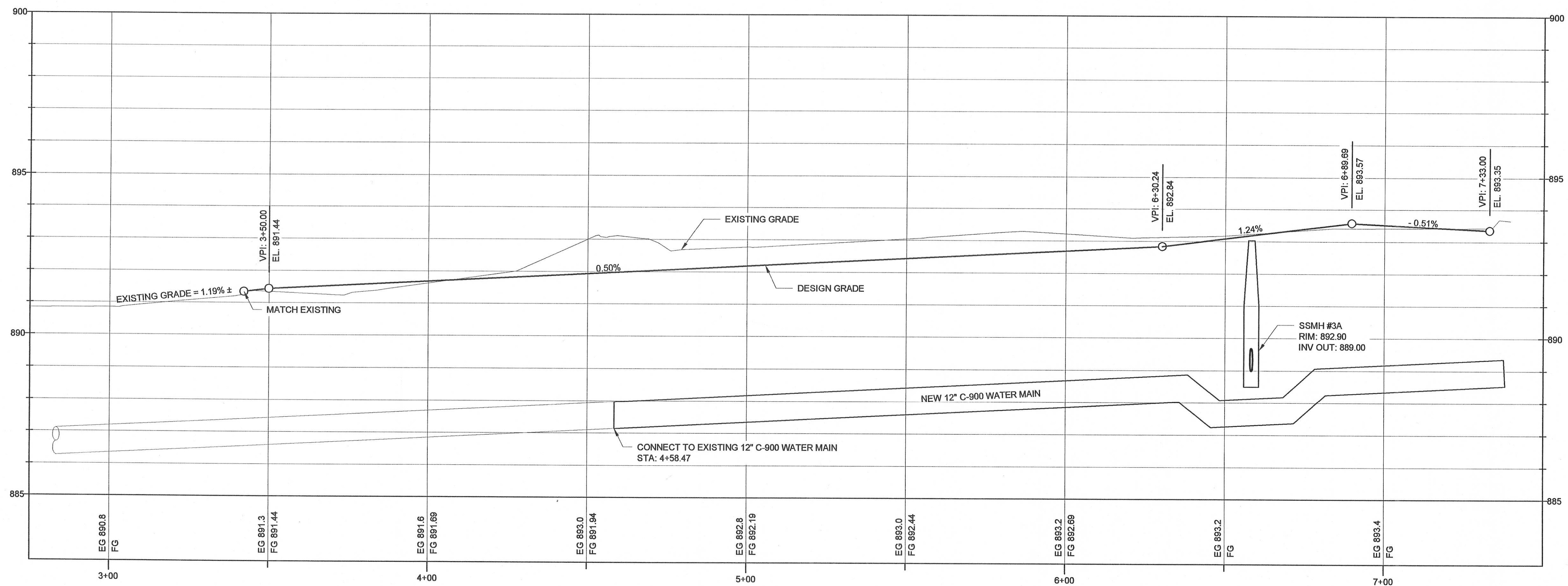
WALL STREET CENTERLINE PROFILE STA: 2+75 - 7+50
