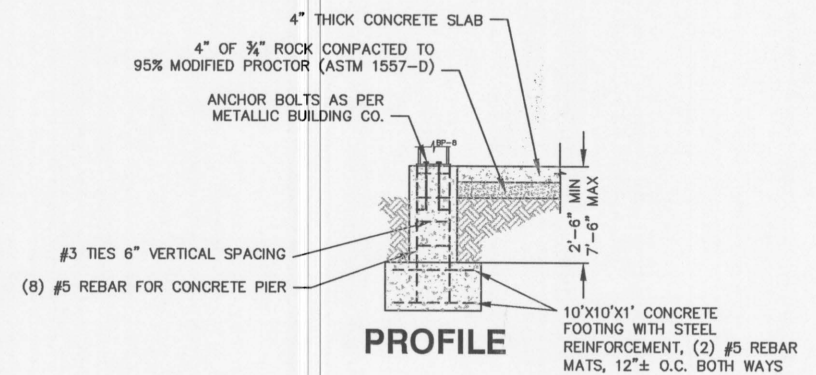
3 FOOTING DETAIL BP-5 OR BP-6 SCALE: 1"=2'
