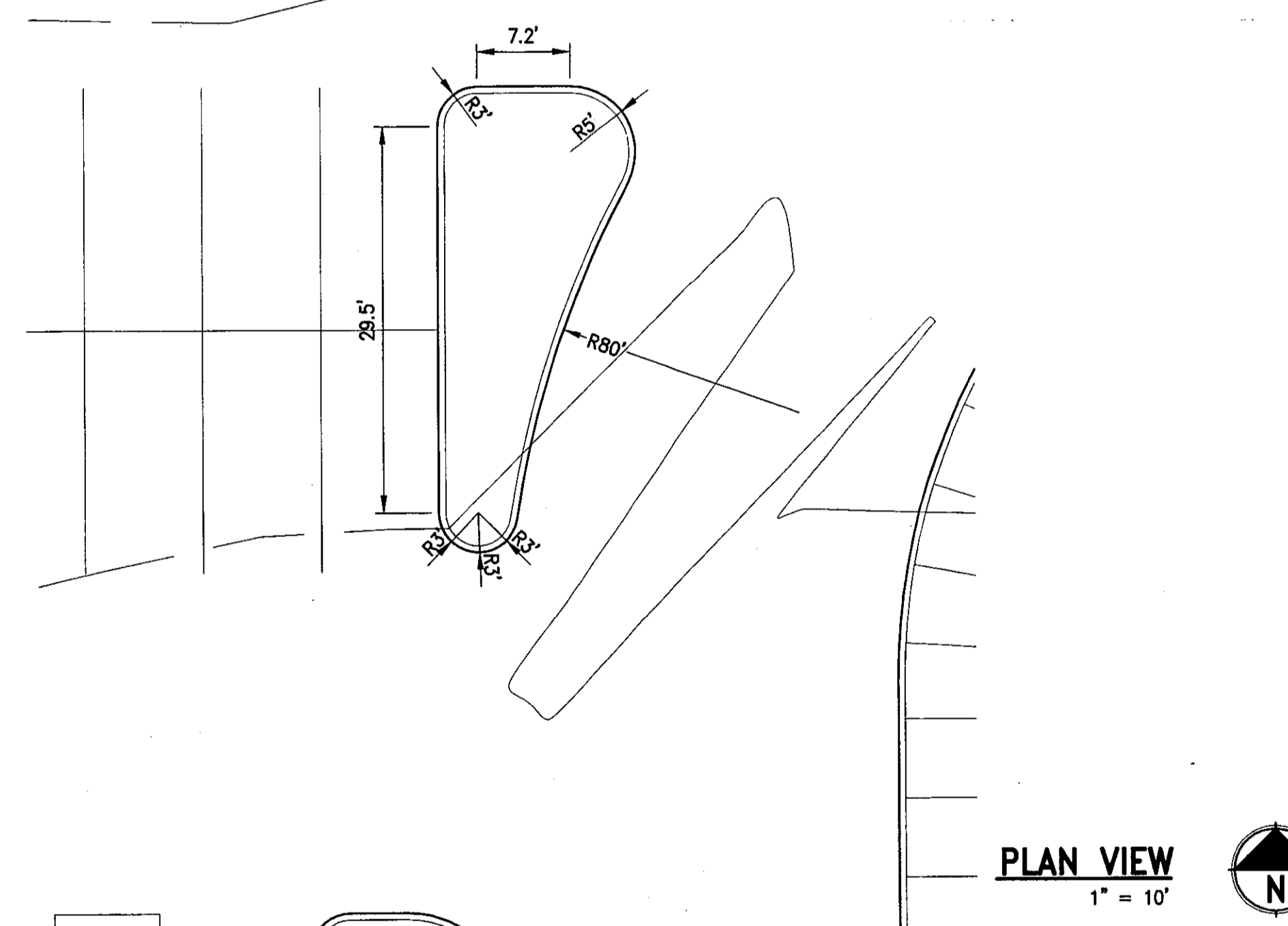
TYPICAL ISLAND DETAILS SCALE: 1" = 10'
