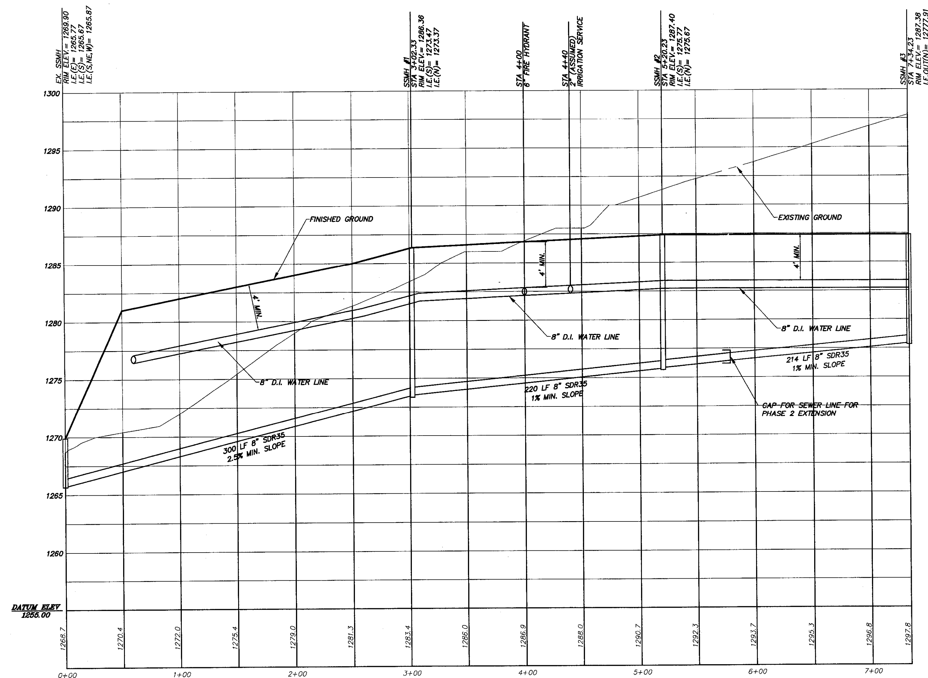
WEST SEWER PROFILE
