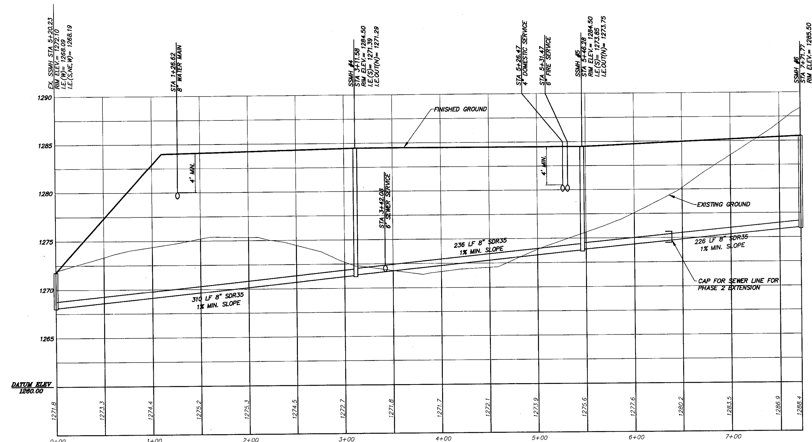
EAST SEWER PROFILE
