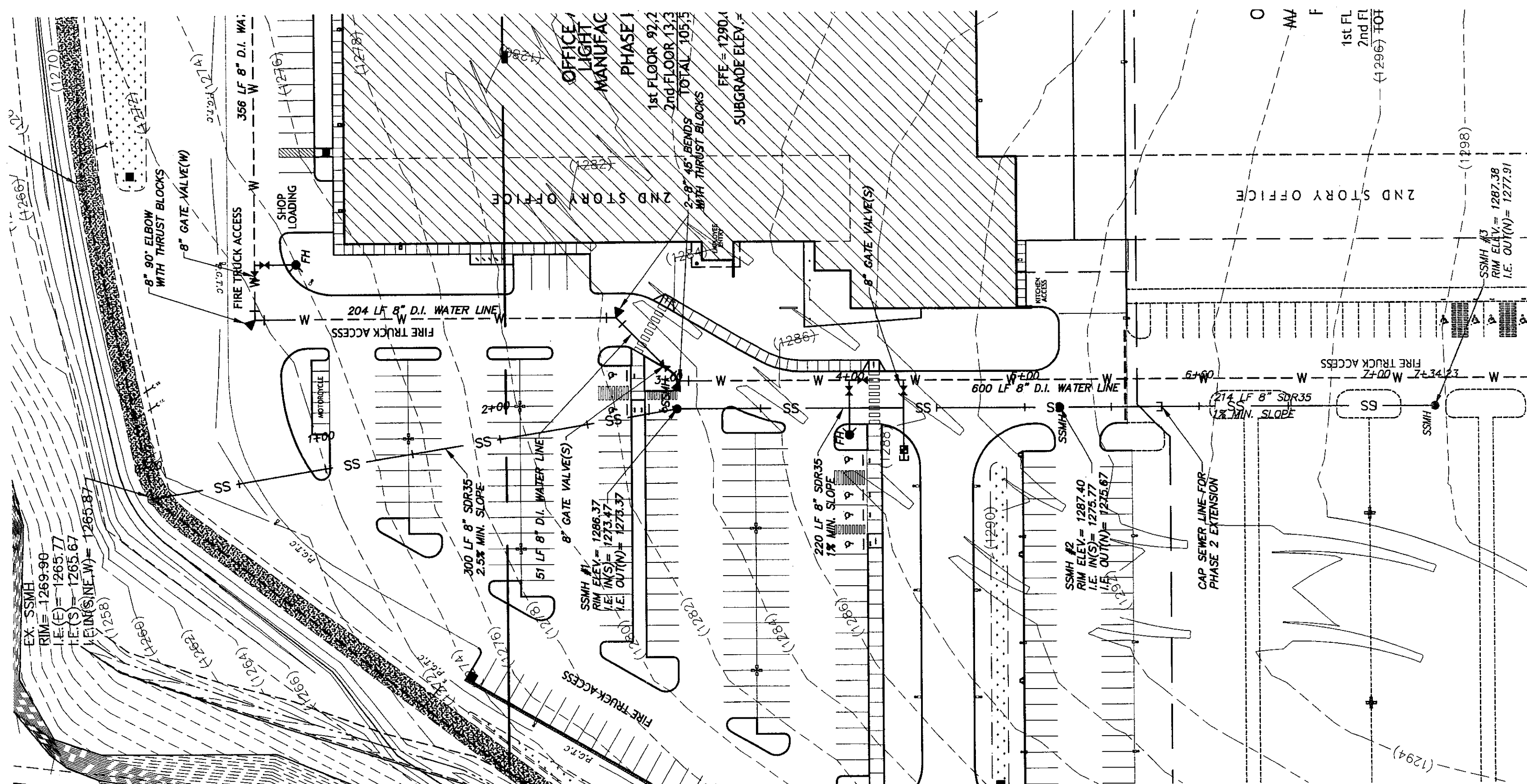
WEST SEWER PLAN
